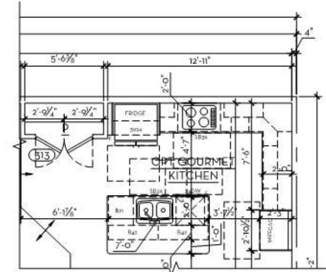
2 UNIT TYPE A6 W/ OPT GOURMET KITCHEN SCALE: 3/8"=1'-0"
